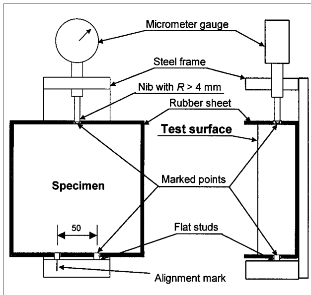
Fig. 4 - Specimen on the three-point expansometer.
