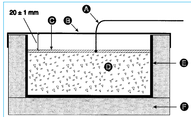
Fig. 7 – Test set-up. A = Thermo-element, B = Evaporation protection, C = Freezing medium, D = Specimen, E = Rubber cloths, F = Thermal insulation.
