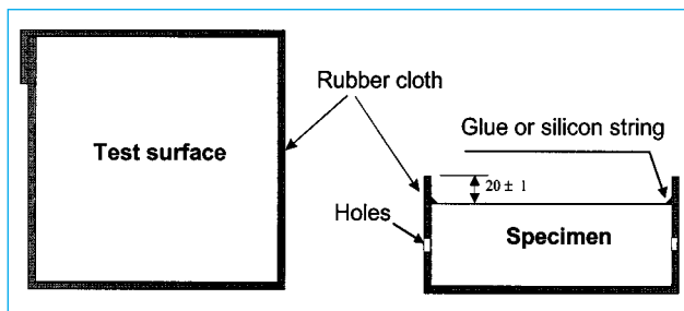
Fig. 3 - Specimen after gluing of rubber cloth (left - a top view, right - a side view).
