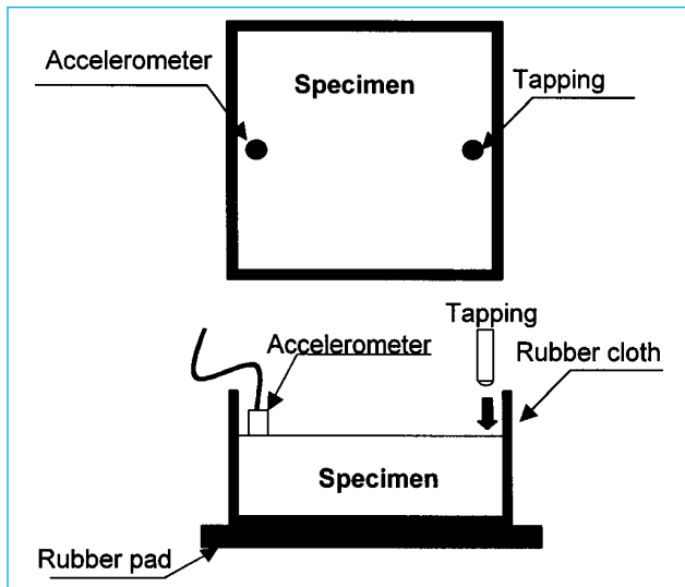
Fig. 6 – Illustration for the FF measurement (upper – a top view, lower – a side view).
