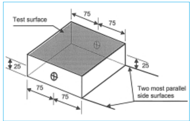
Fig. 2b - Illustration of the marks for the alternative procedure A.
