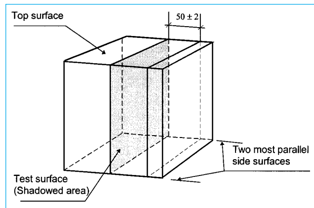
Fig. 1 – Illustration of sawing of a specimen.
