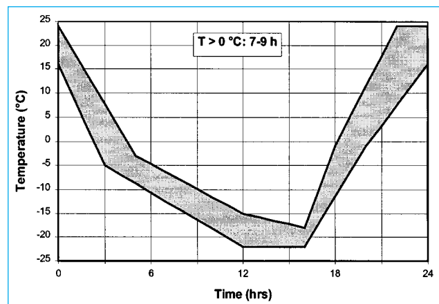
Fig. 8 – Temperature regime for one cycle of freezing-and-thawing. The temperature in the freezing medium at the centre of the test surface shall be within the shaded area and shall exceed 0^\circ\text{C} for at least 7 hours but no more than 9 hours during each cycle.
