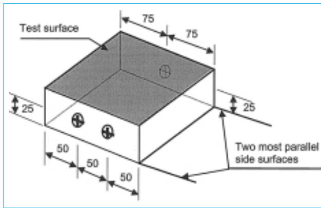
Fig. 2a - Illustration of the marks for the reference procedure.
