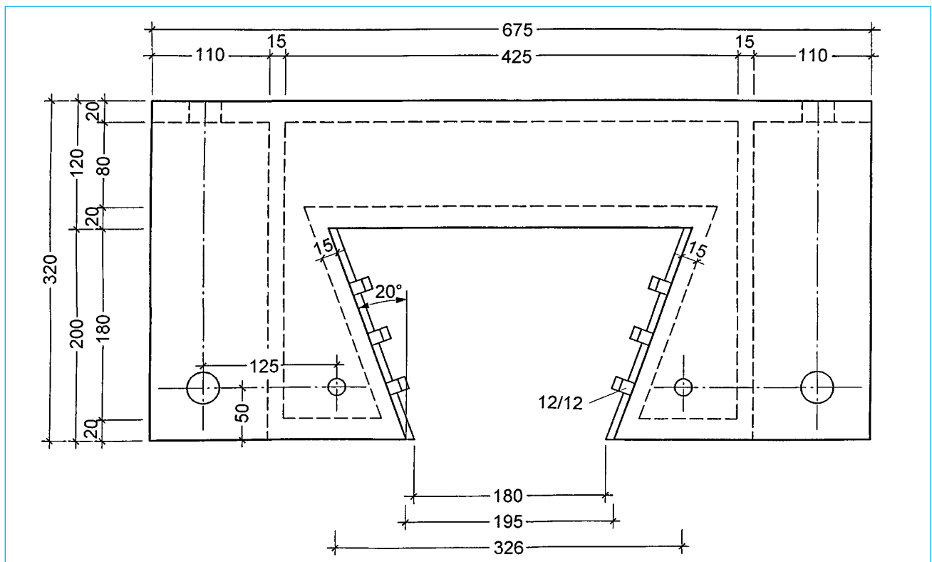
Fig. 2a - Cross-head: Detail plan.
